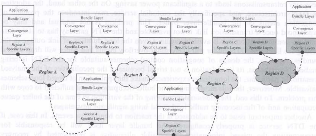
Figure 10. DTN protocol architecture.
