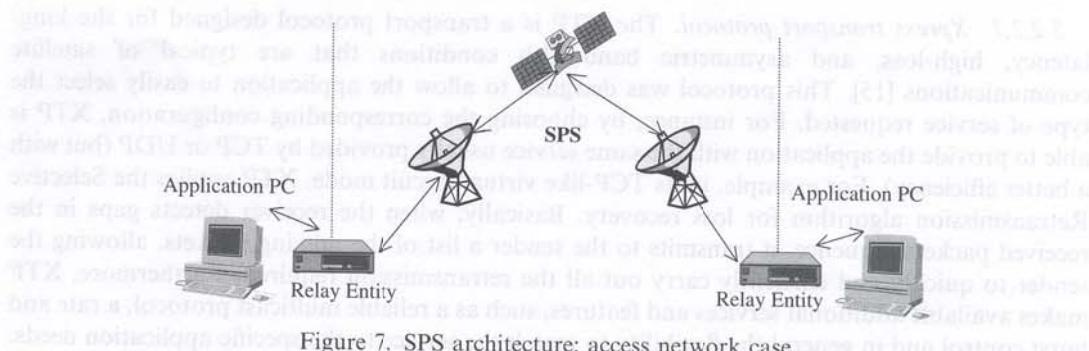
Figure 7. SPS architecture; access network case.
